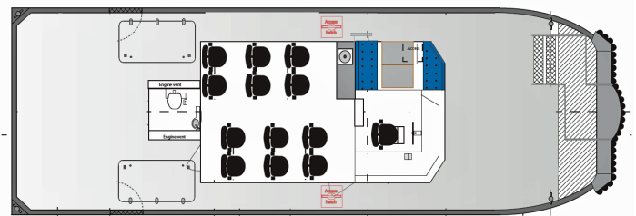
Fastnet Shipping Ltd Fastnet Skua & Fastnet Puffin GA Plan
